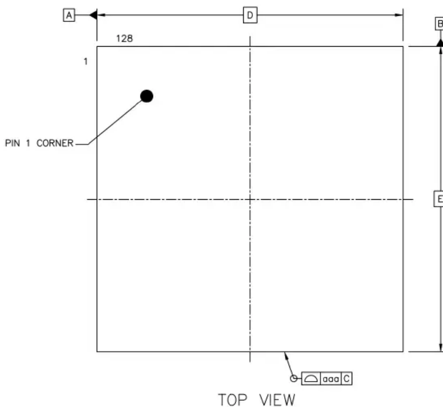
Fig.2-3 Package Top View
