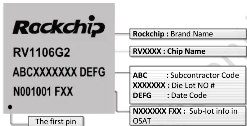
Fig.2-1 RV1106G2 Package definition
