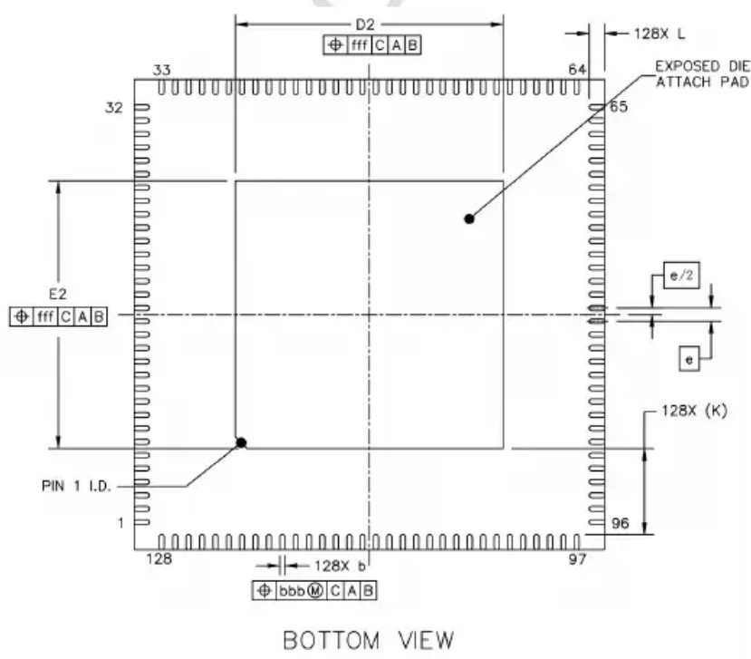
Fig.2-4 Package Bottom View
