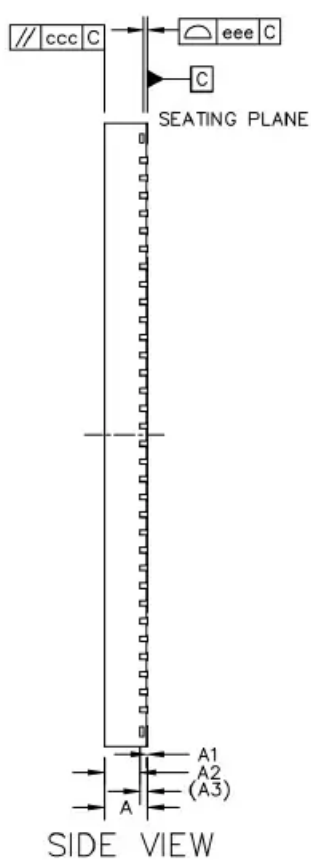
Fig.2-4 Package Side View
