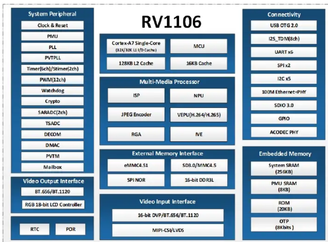
Fig.1-1 Block Diagram
