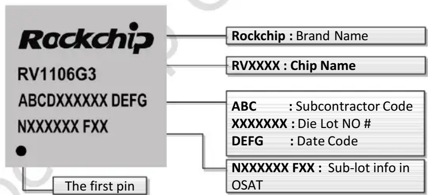
Fig.2-2 RV1106G3 Package definition
